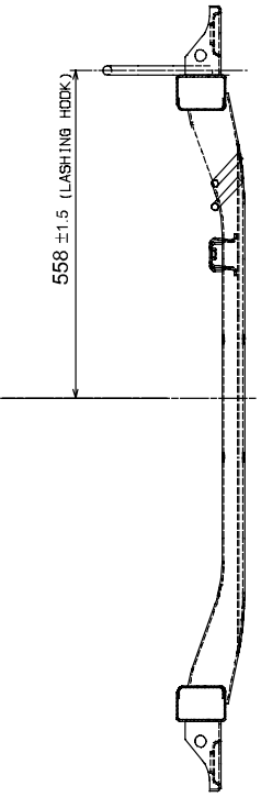
SECTION C
