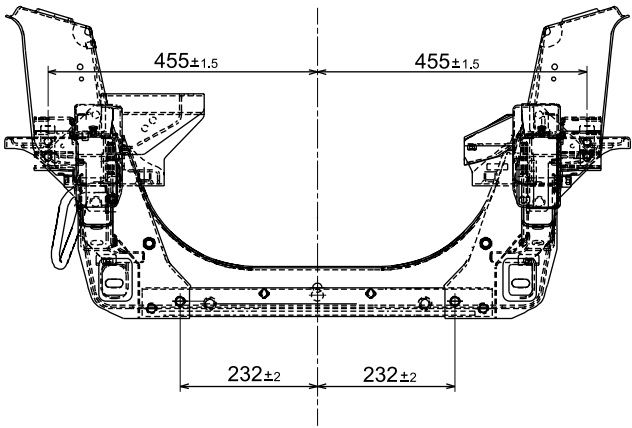
SECTION B
