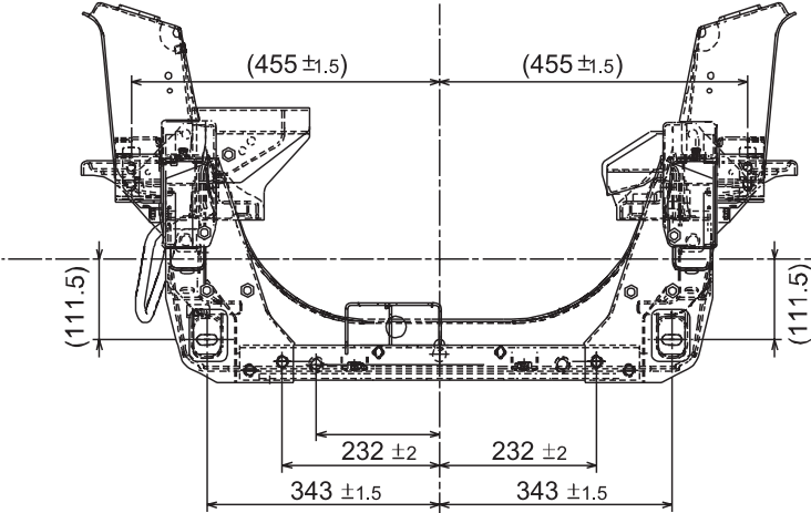
SECTION B
