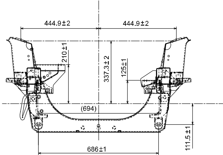
SECTION A
